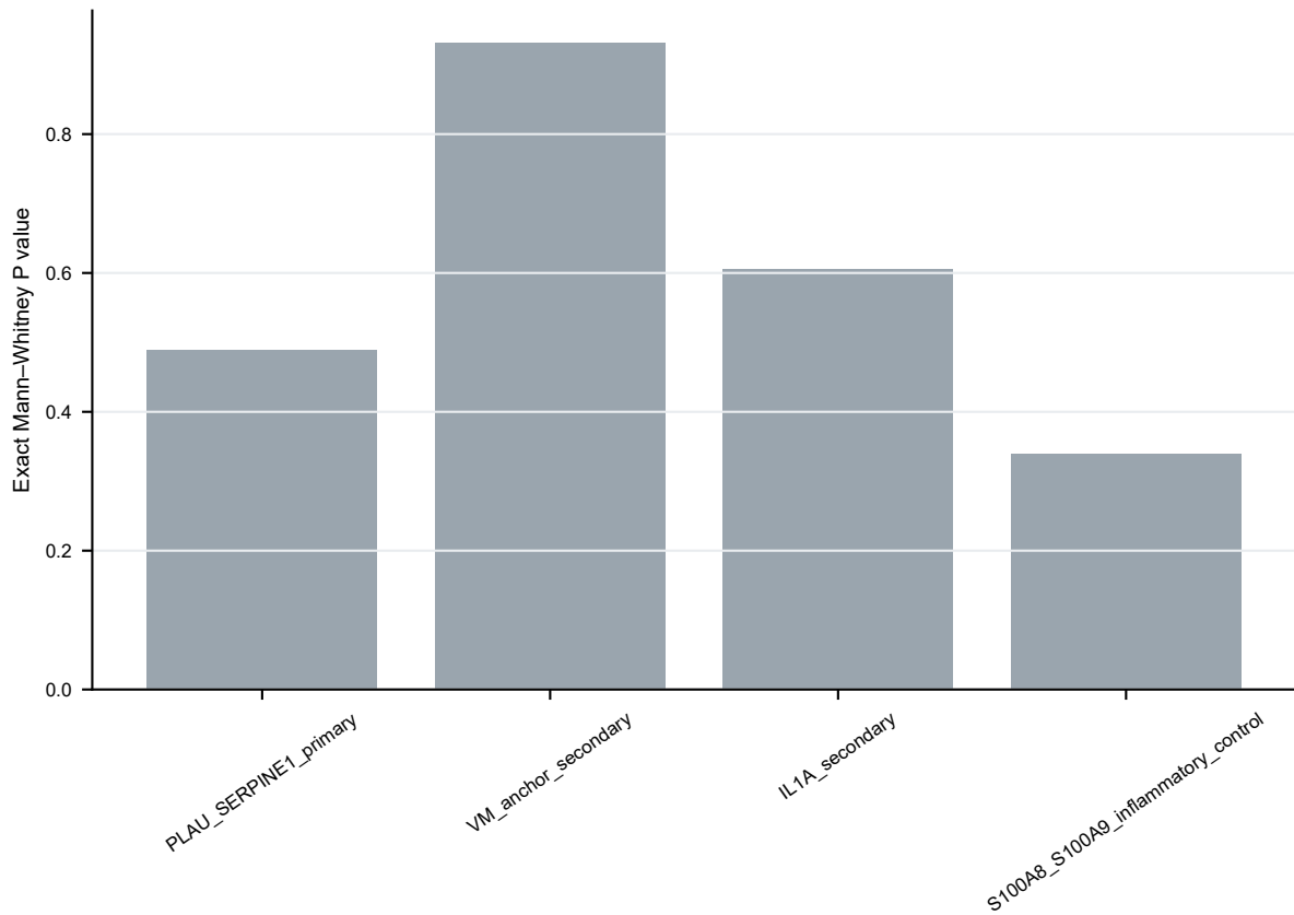
Fig. S11 | GSE255058 treatment-response negative audit
