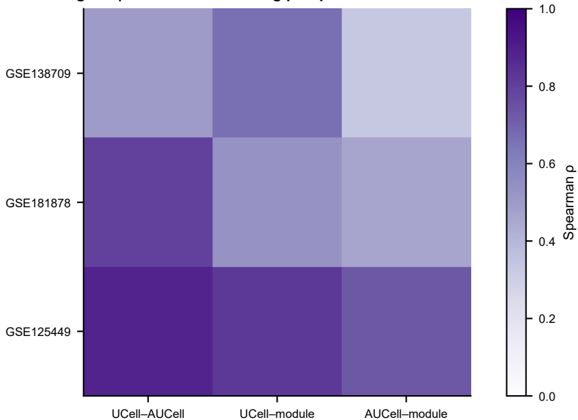
Fig. S2 | Concordance among prespecified VM-like scores
