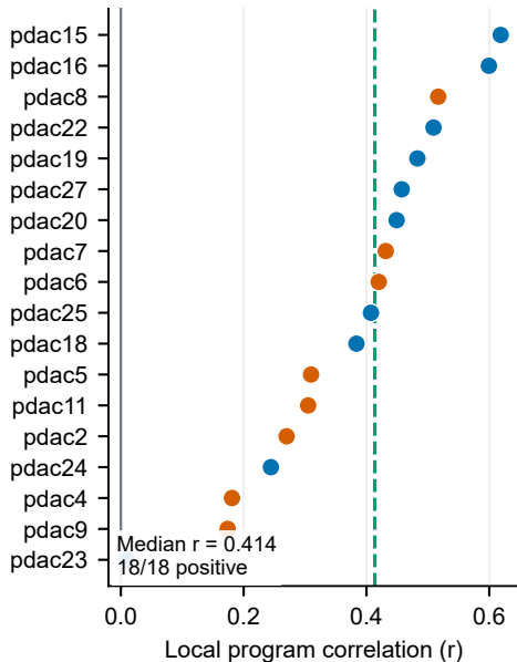
GSE277116: sample-level technical replication
