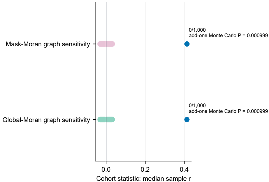
GSE277116: sample-level technical replication
