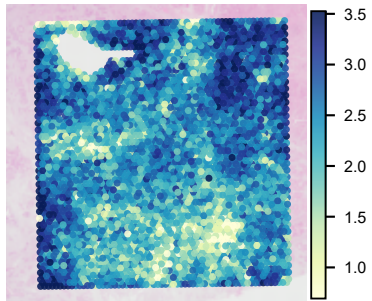
DC-core score
