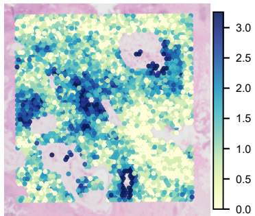
DC-core score
