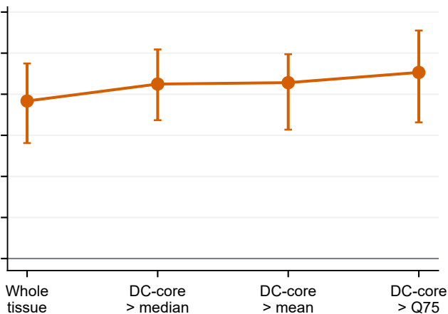
GSE277116: with DC-core residualization
