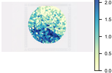
DC-core score
