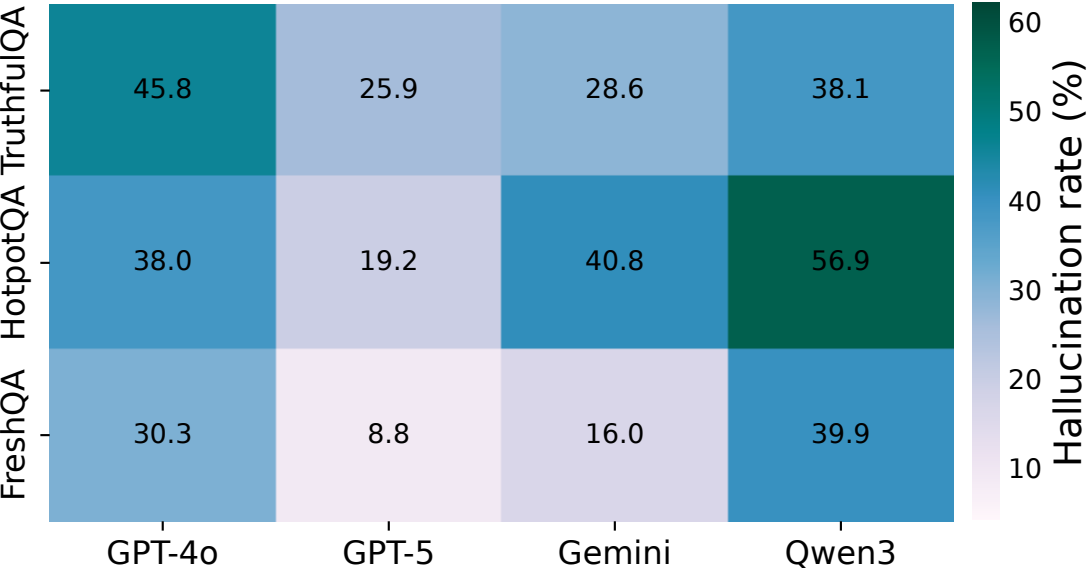
Hallucination Rates Heatmap Overview
