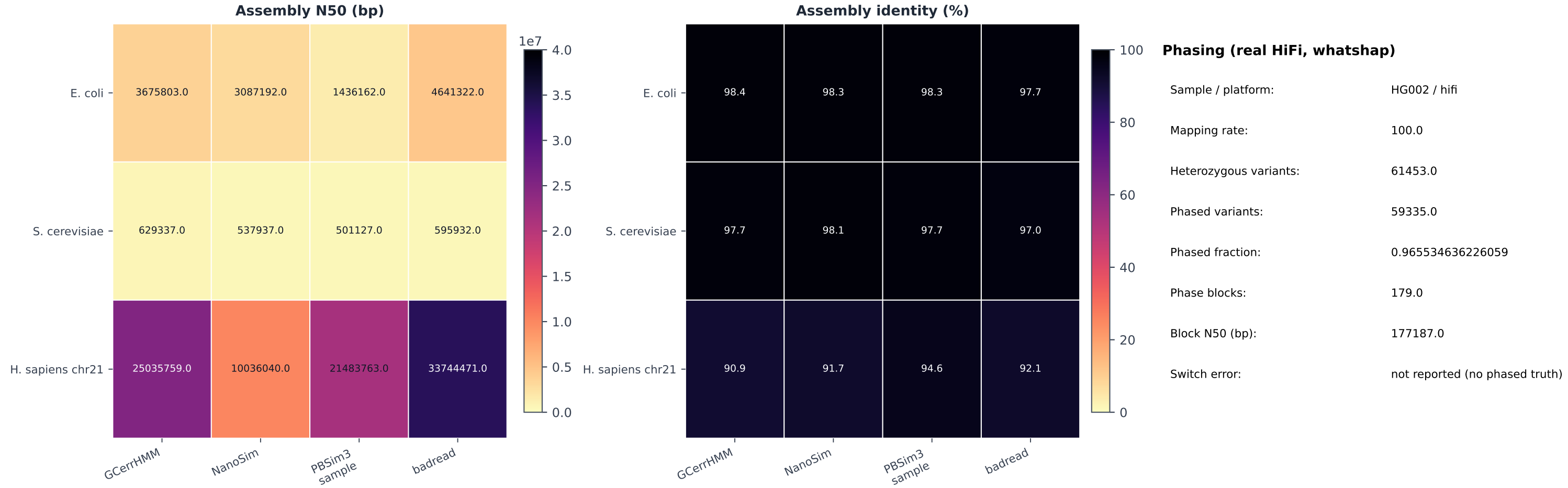
Figure 5. Assembly (Flye for ONT, hifiasm for HiFi) and phasing
