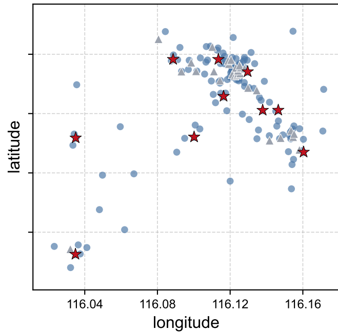
Skewed Density CV = 0.600
