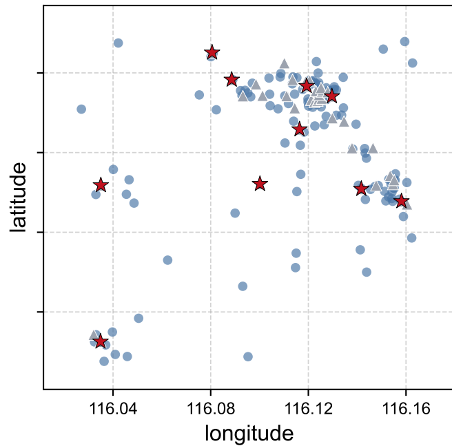
Clustered Density CV = 0.534
