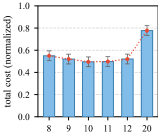
(a) Number of edge servers.
