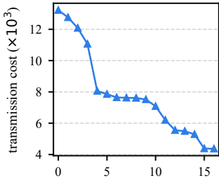
(b) Convergence behavior.
