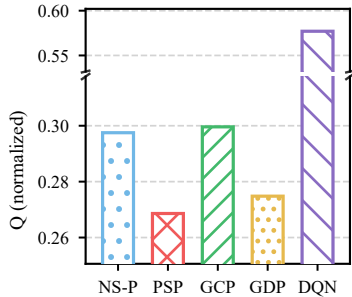
(a) # users (100).
