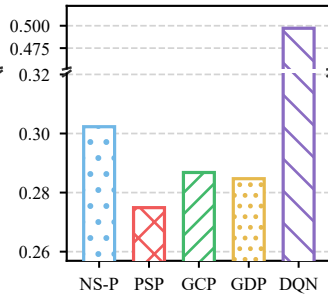
(c) # users (150).
