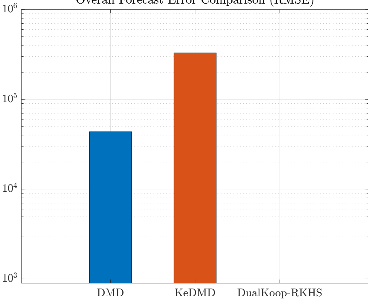
Overall Forecast Error Comparison (RMSE)
