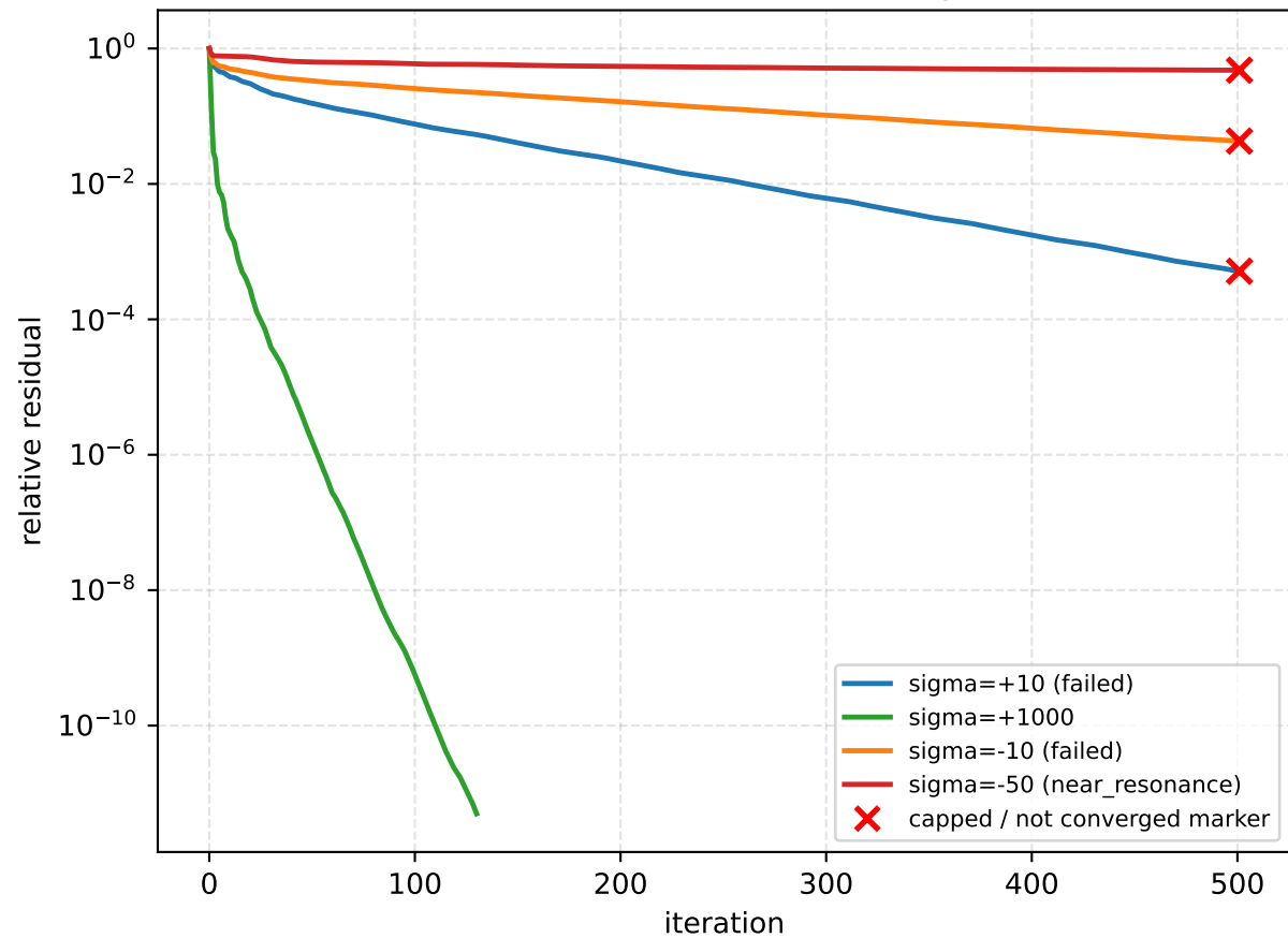
(b) Relative residual history
