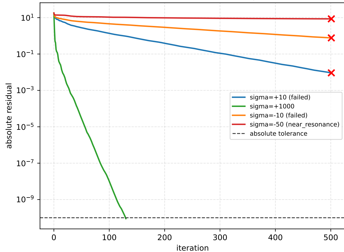
(a) Absolute residual history
