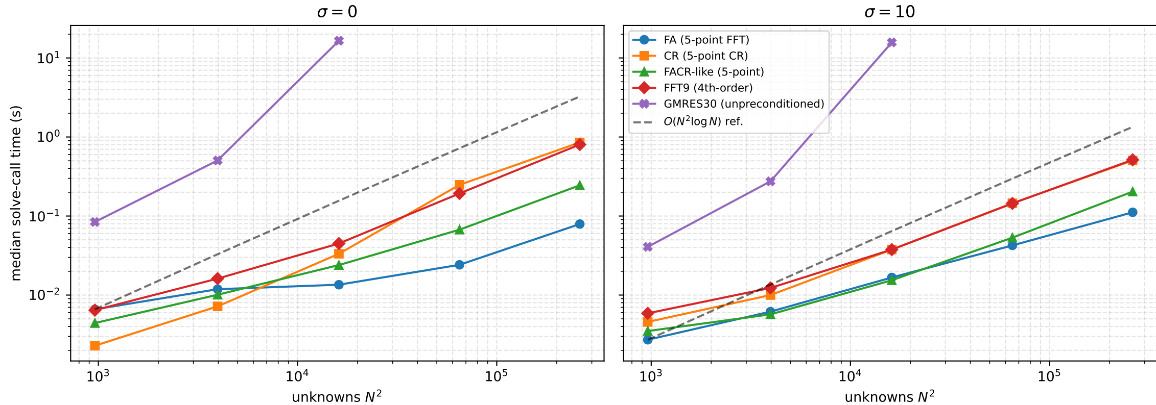
Time scaling of current implementations
