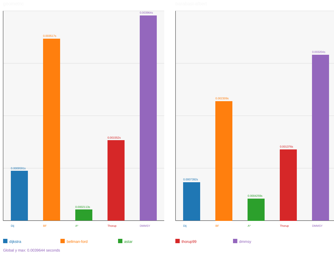
Figure 1: Median runtime by algorithm on the deterministic geometric and Barabási–Albert benchmark profiles (seed 2026, one recorded repeat, setup and file IO excluded). Thorup uses the documented integer-undirected graph view. Detailed samples, IQRs, fingerprints, and DMMSY/Dijkstra ratios are recorded in bench/results/sssp-benchmark-seed-2026.csv .
