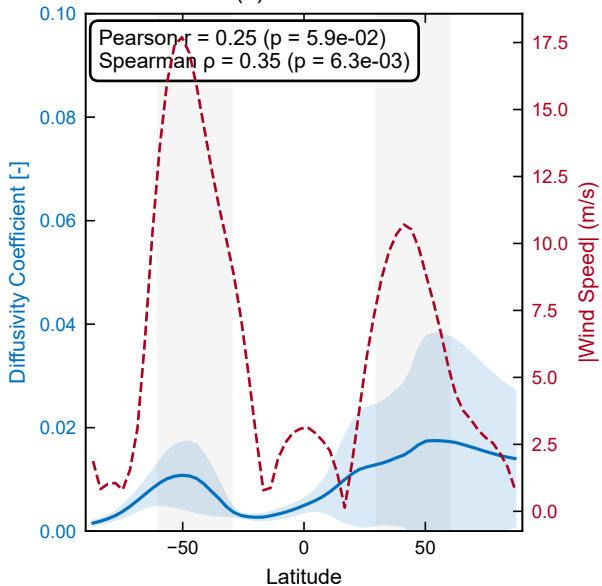
(a) Holocene
