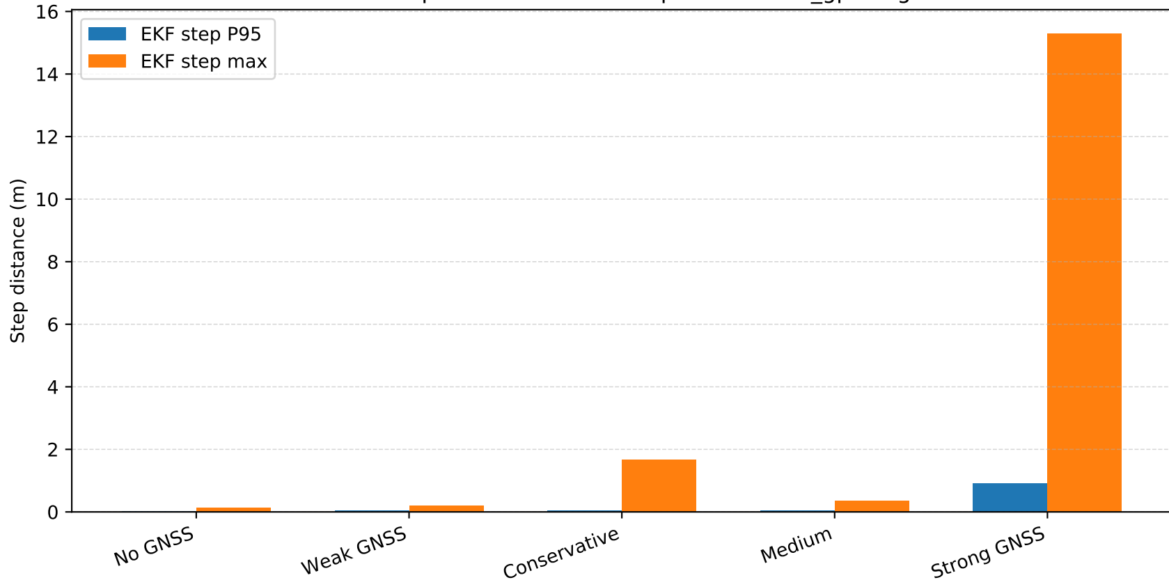
EKF Output Smoothness Comparison on all_gps.bag
