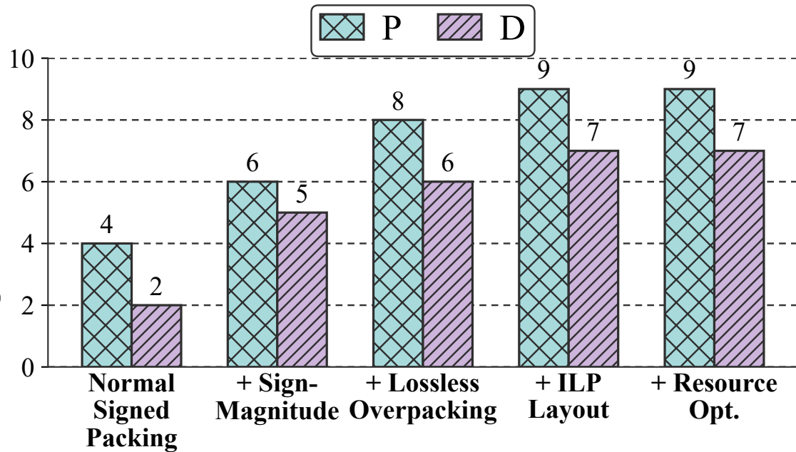
Packing Number Per DSP
