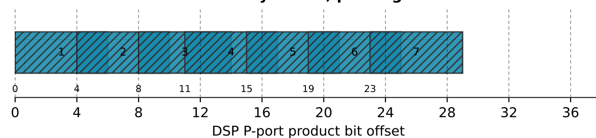
+ ILP Layout - D, packing=7
