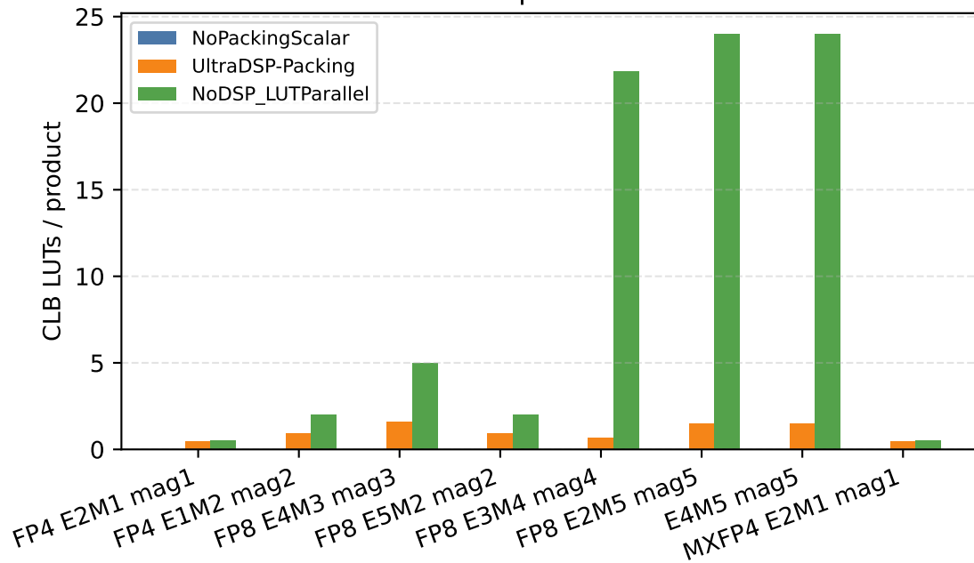
C. LUT per Product
