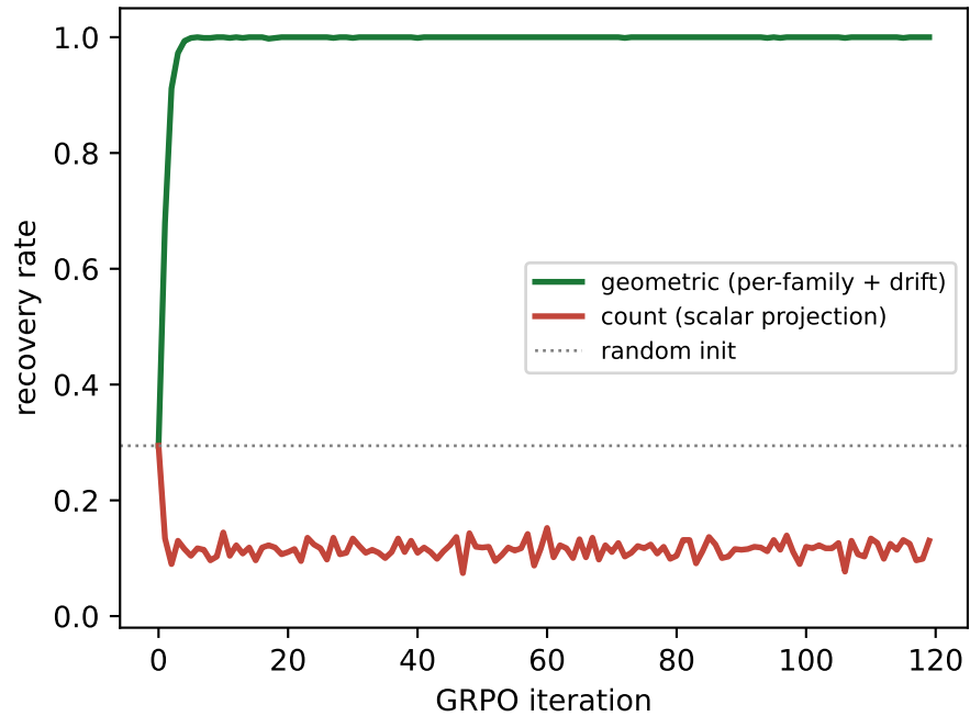
(a) coupled \sigma -het trap: training curve
