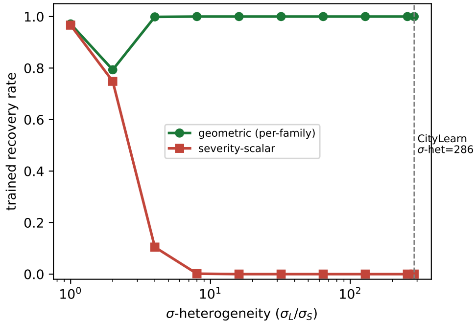
(b) trained recovery vs \sigma -heterogeneity
