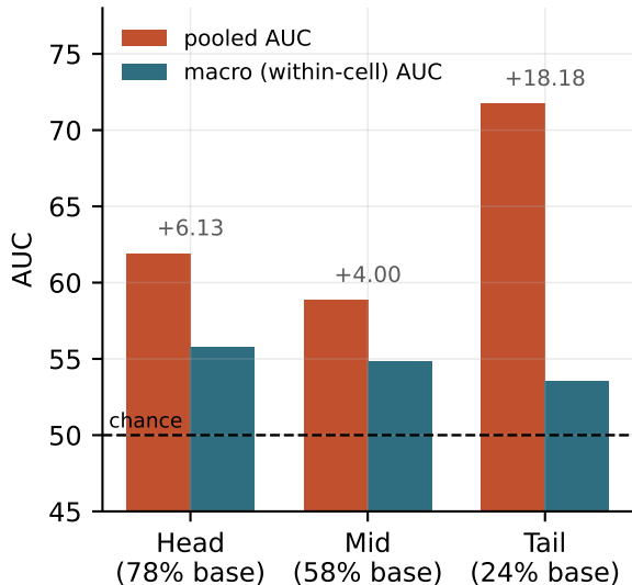
Pooling flatters the model most in the sparsest region
