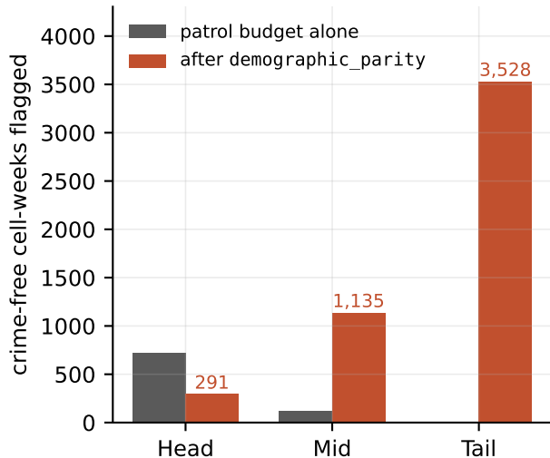
The remedy moves attention to where the model has least skill
