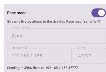
Android — Race mode card
