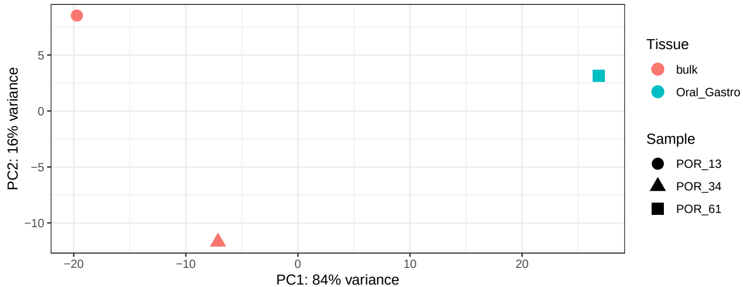
PCA of VST-transformed counts
