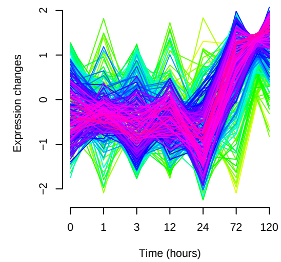
Cluster 4
