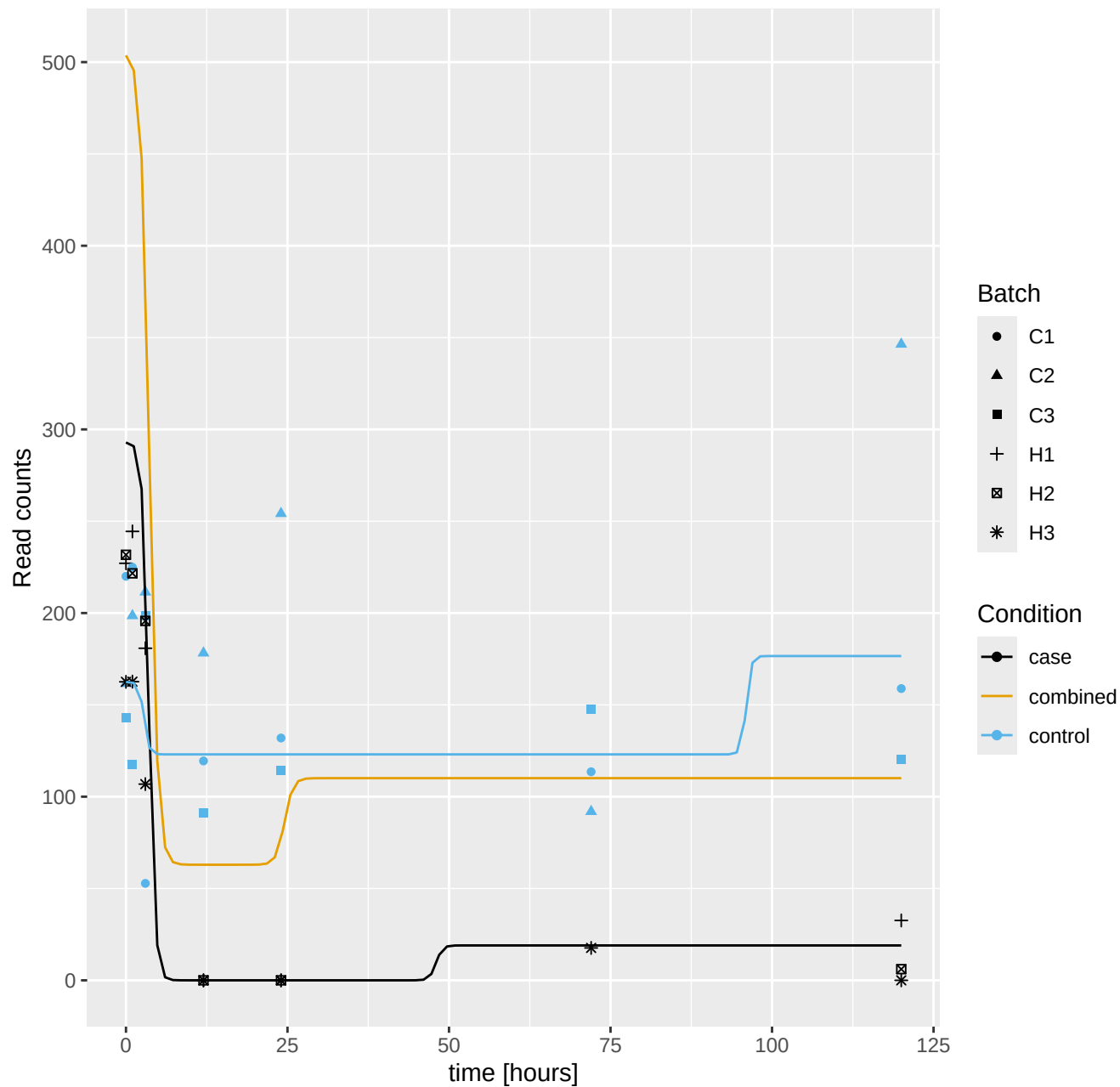
Montipora_capitata_Hlv3___TS.g49643.t1: log10 q = -26.58
