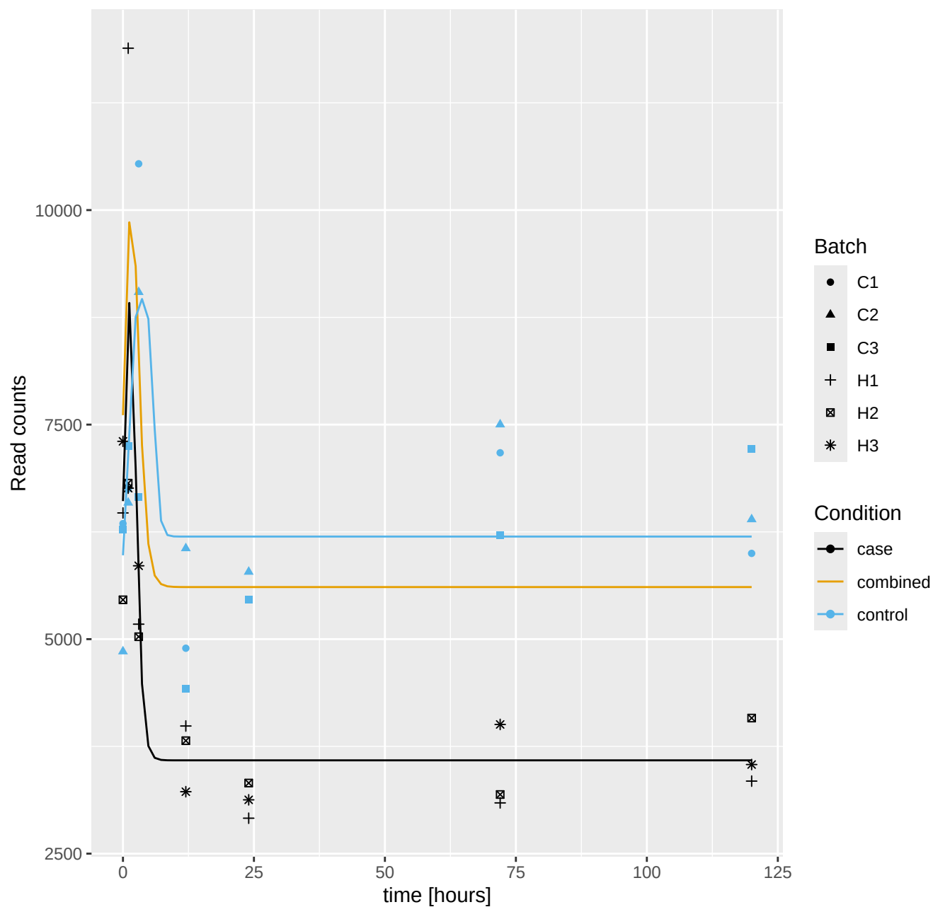
Pocillopora acuta Hlv2 RNAseq.g11741.t1: log10 q = -5.86
