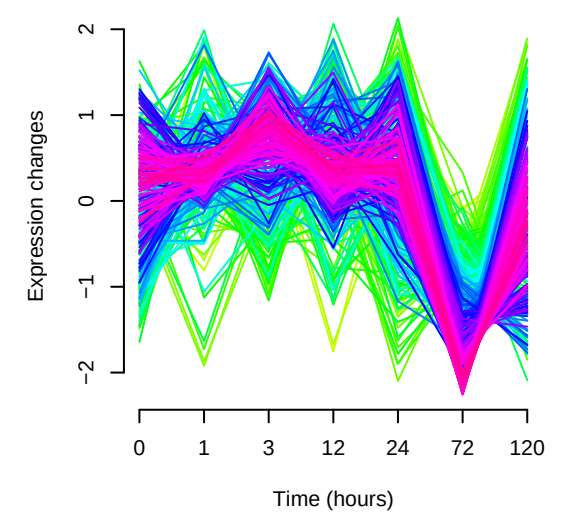
Cluster 4
