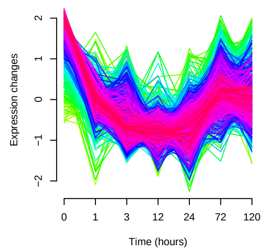
Cluster 3
