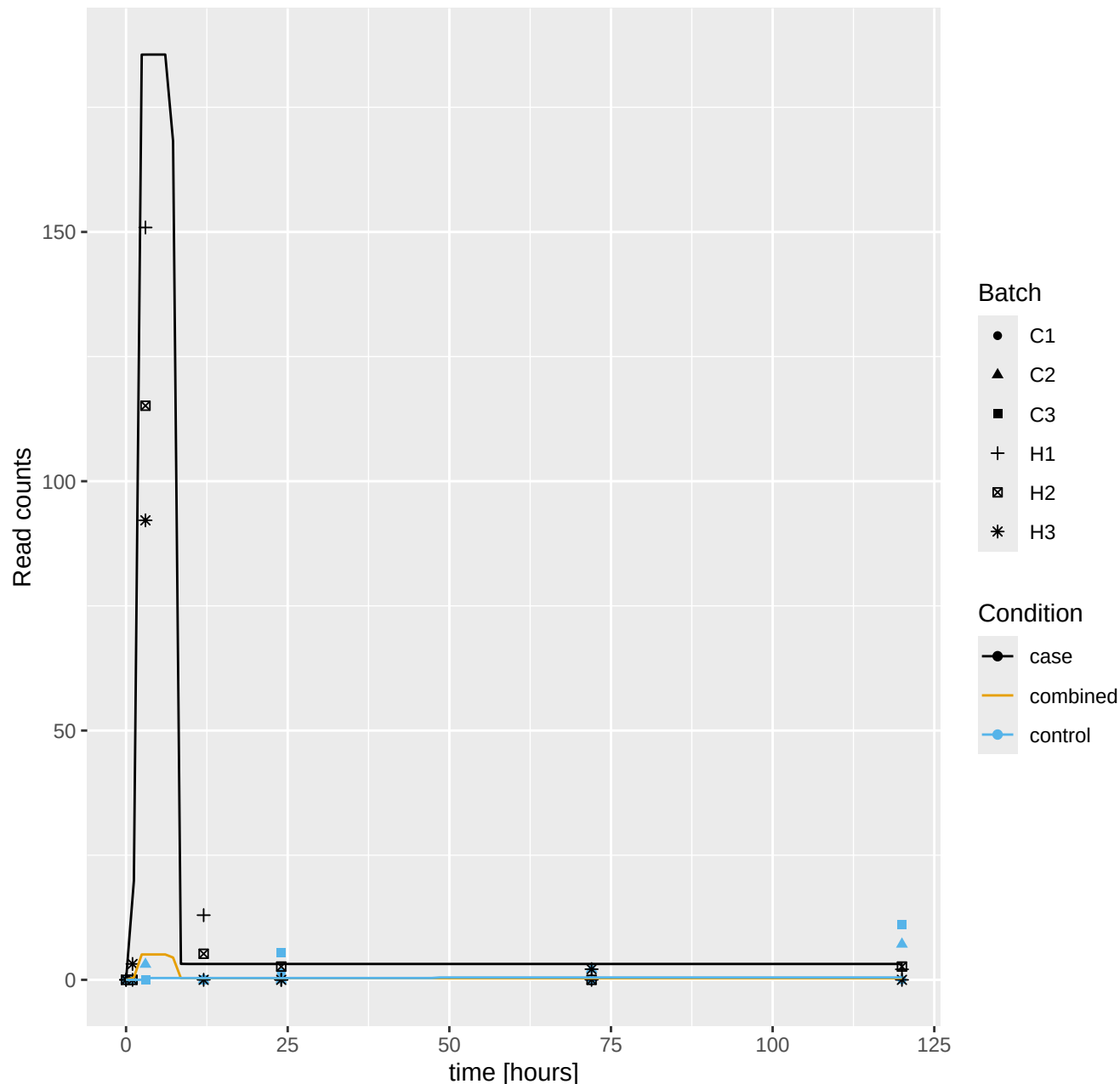
Porites_compressa_Hlv1____RNAseq.g39940.t1: log10 q = 0
