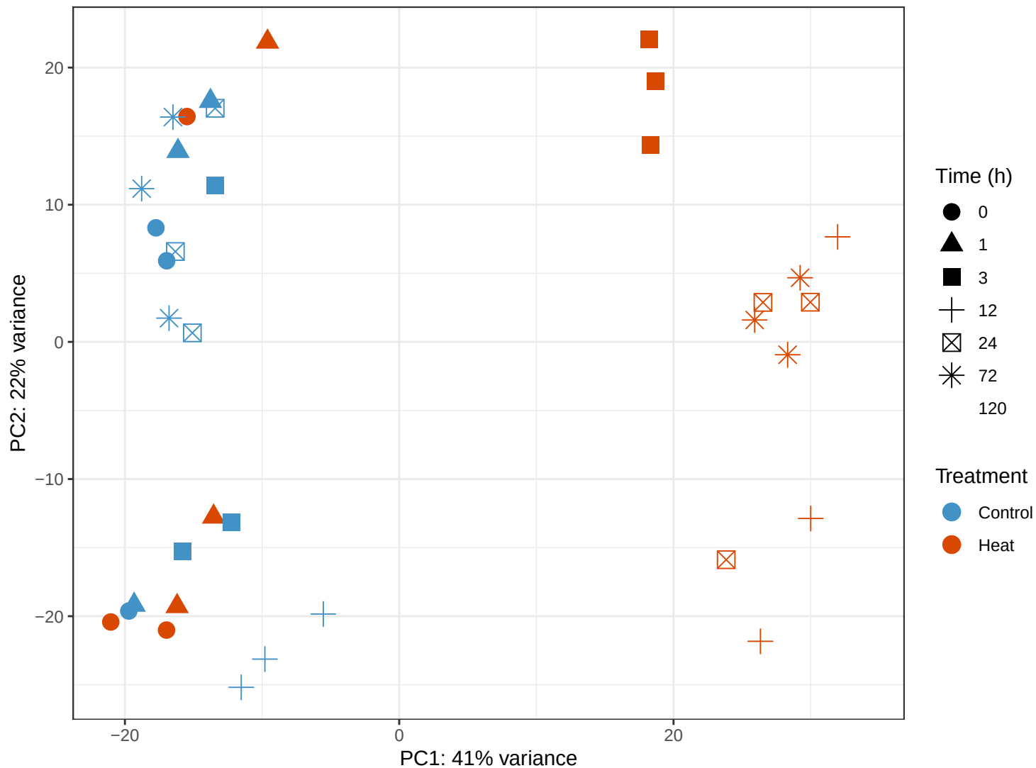
Pacuta – PCA of VST-transformed counts
