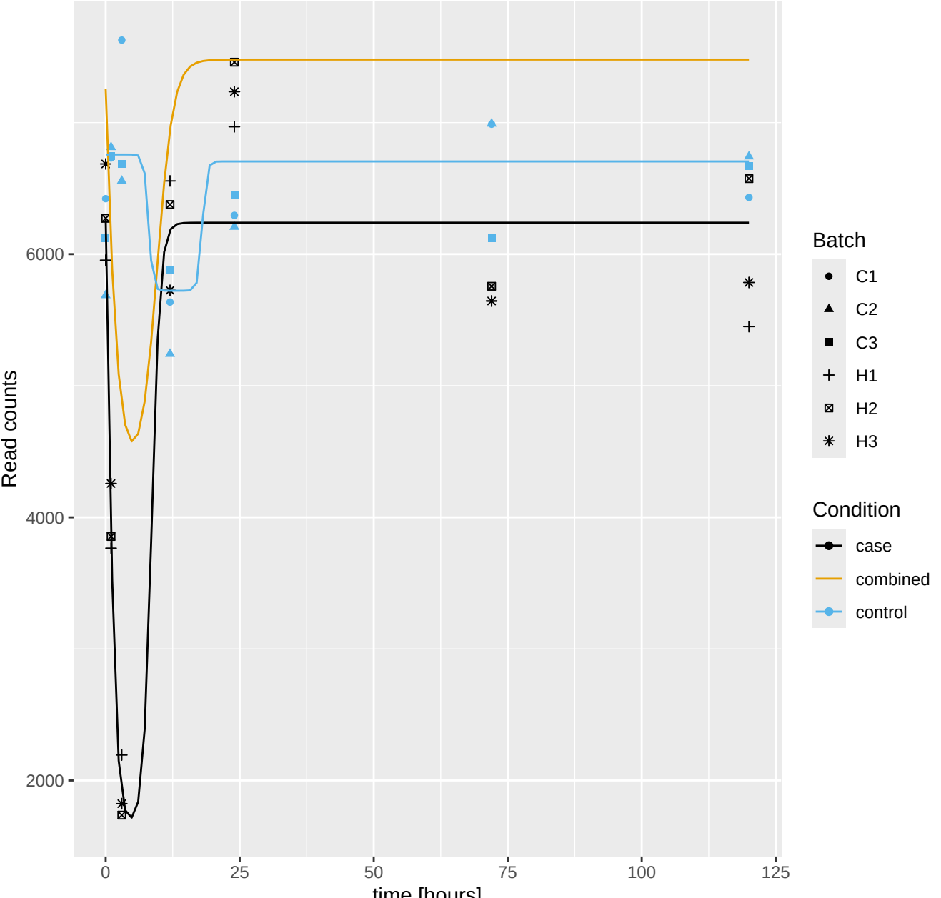
Pocillopora_acuta_Hlv2____RNAseq.g18469.t1: log10 q = -74.9
