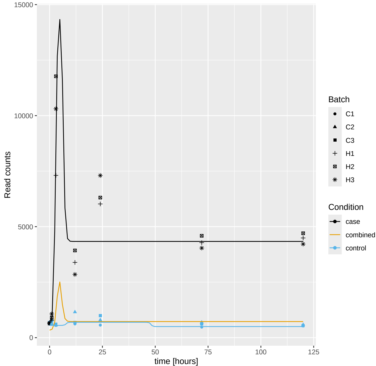
Pocillopora_acuta_Hlv2____RNAseq.g22728.t1: log10 q = -76.93
