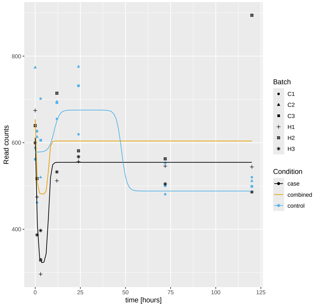
Pocillopora acuta Hlv2 TS.g10300.t1: log10 q = -4.24
