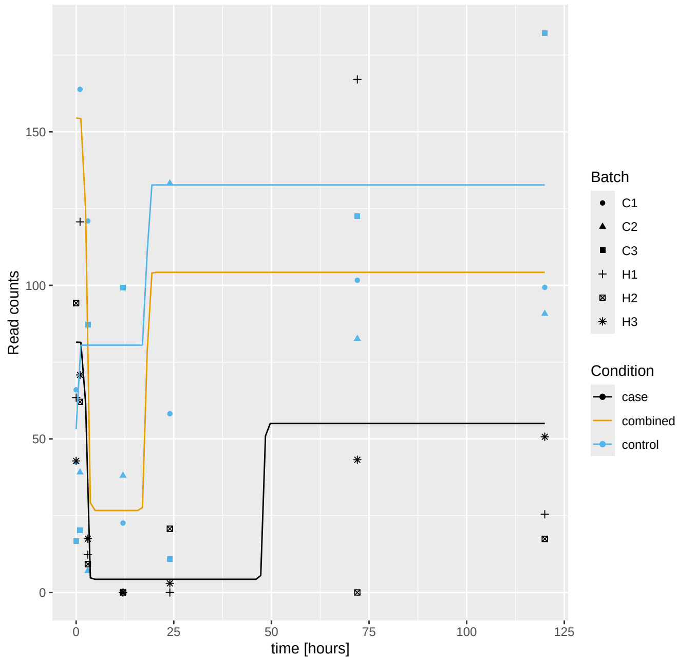
Porites_compressa_Hlv1___TS.g5240.t1: log10 q = -1.36
