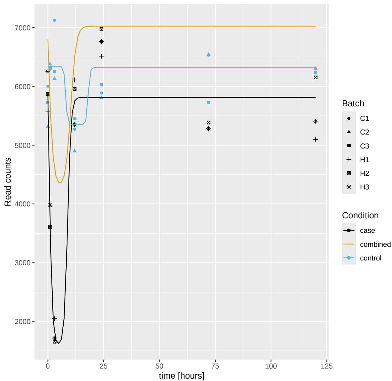
Pocillopora_acuta_Hlv2___RNAseq.g18469.t1: log10 q = -78.66
