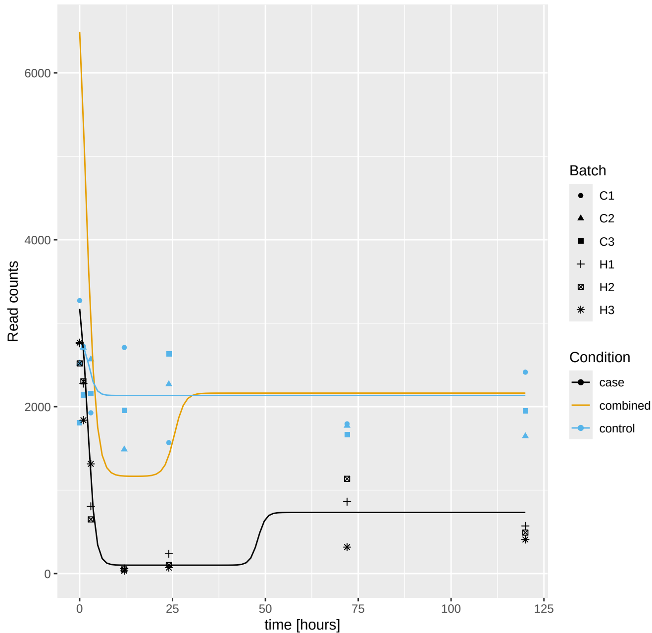
Porites_compressa_Hlv1____RNAseq.g40324.t1: log10 q = -23.89
