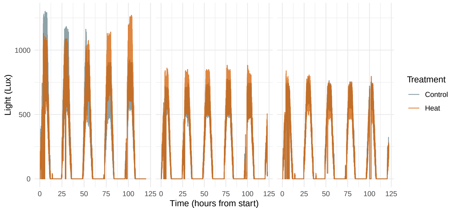
Porites compressa
