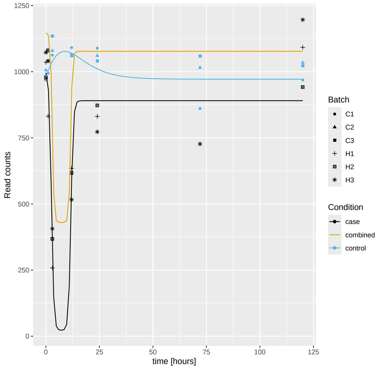
Montipora_capitata_Hlv3___RNAseq.g37139.t1: log10 q = -25.39
