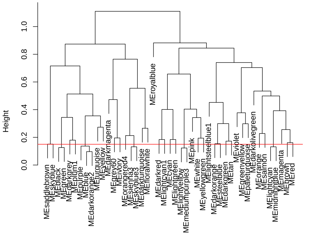
Clustering of module eigengenes (dissimilarity calc = MEDiss = 1–cor(ME
