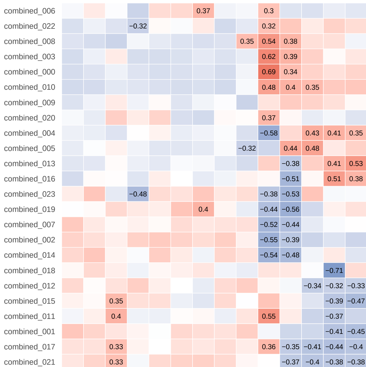
Module-trait Relationships
