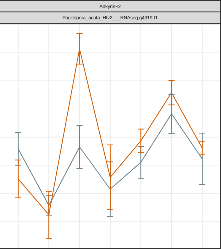
Cluster 4
