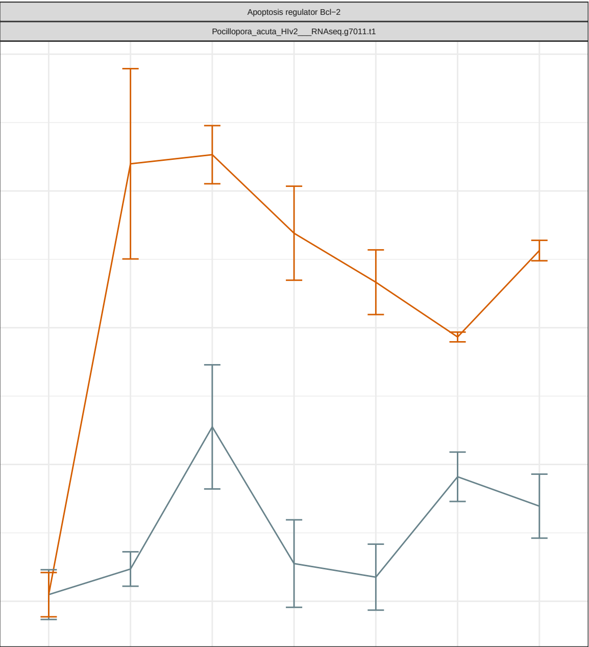
Cluster 3
