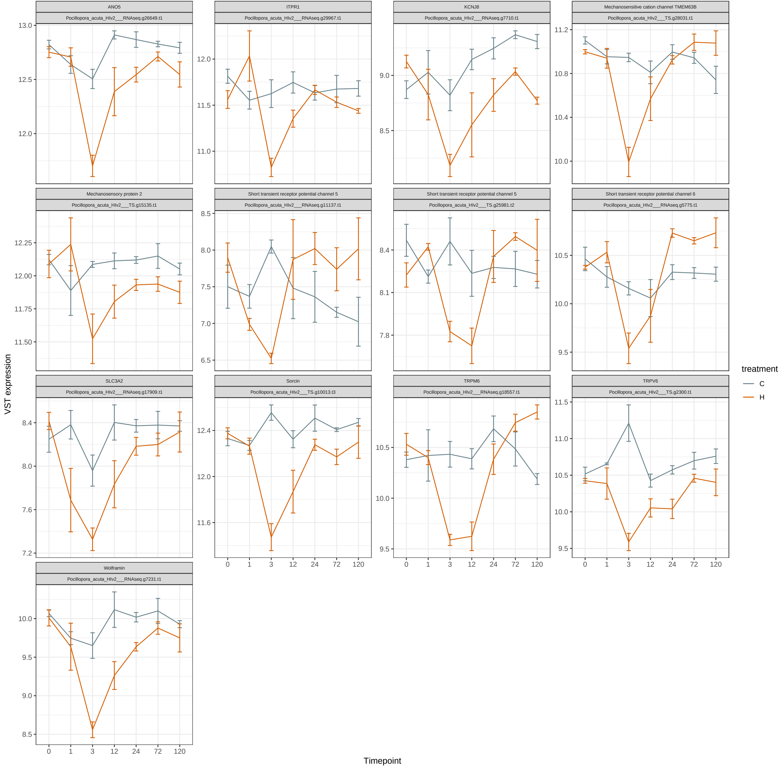
Cluster 2
