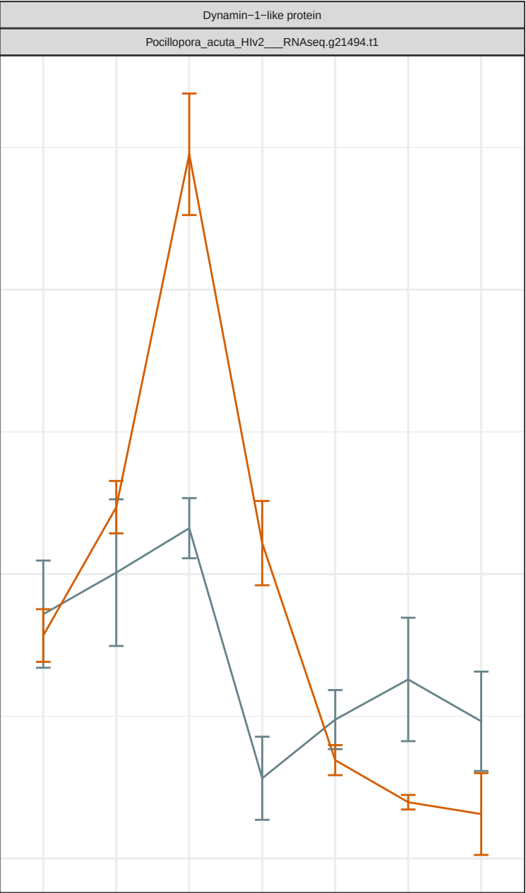
Cluster 6
