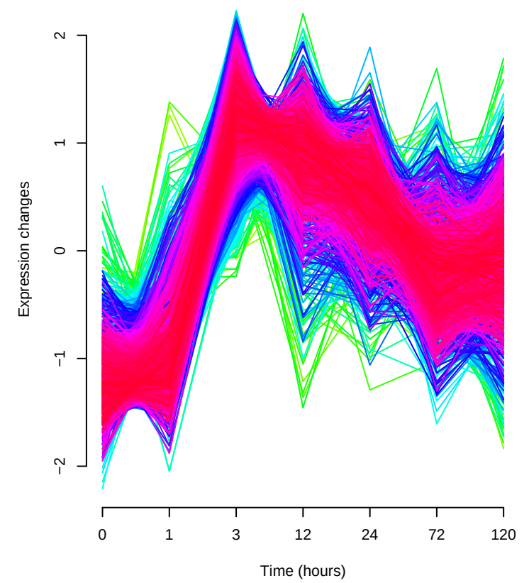
Cluster 6
