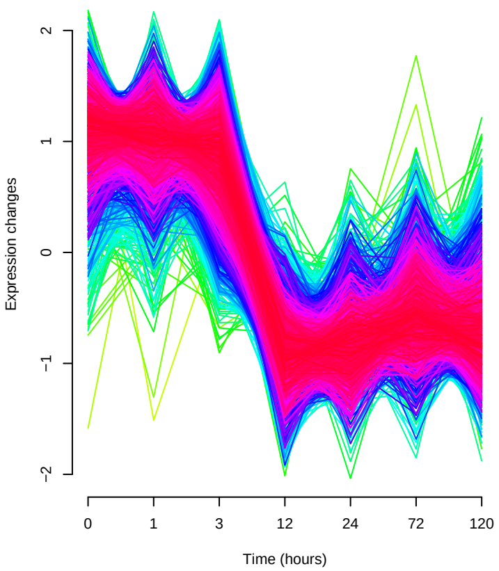
Cluster 4
