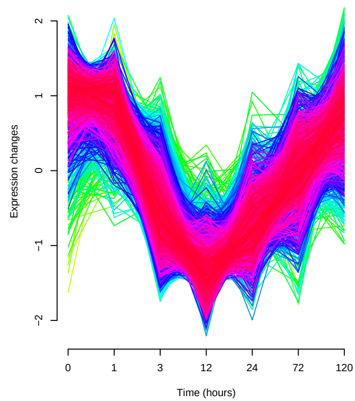
Cluster 5
