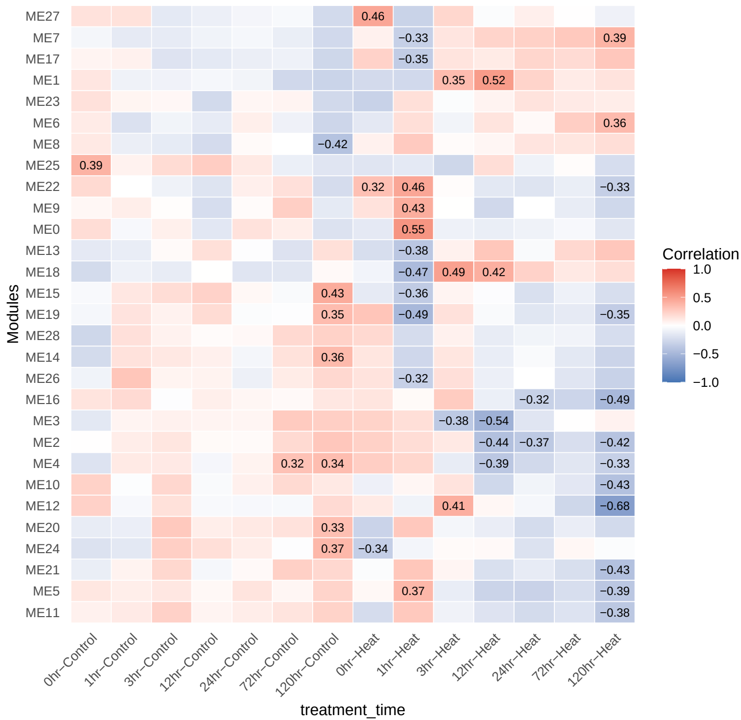
Module-trait Relationships
