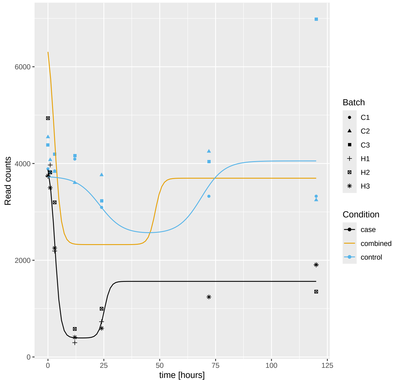
Montipora_capitata_Hlv3__RNAseq.g26807.t1: log10 q = -25.29
