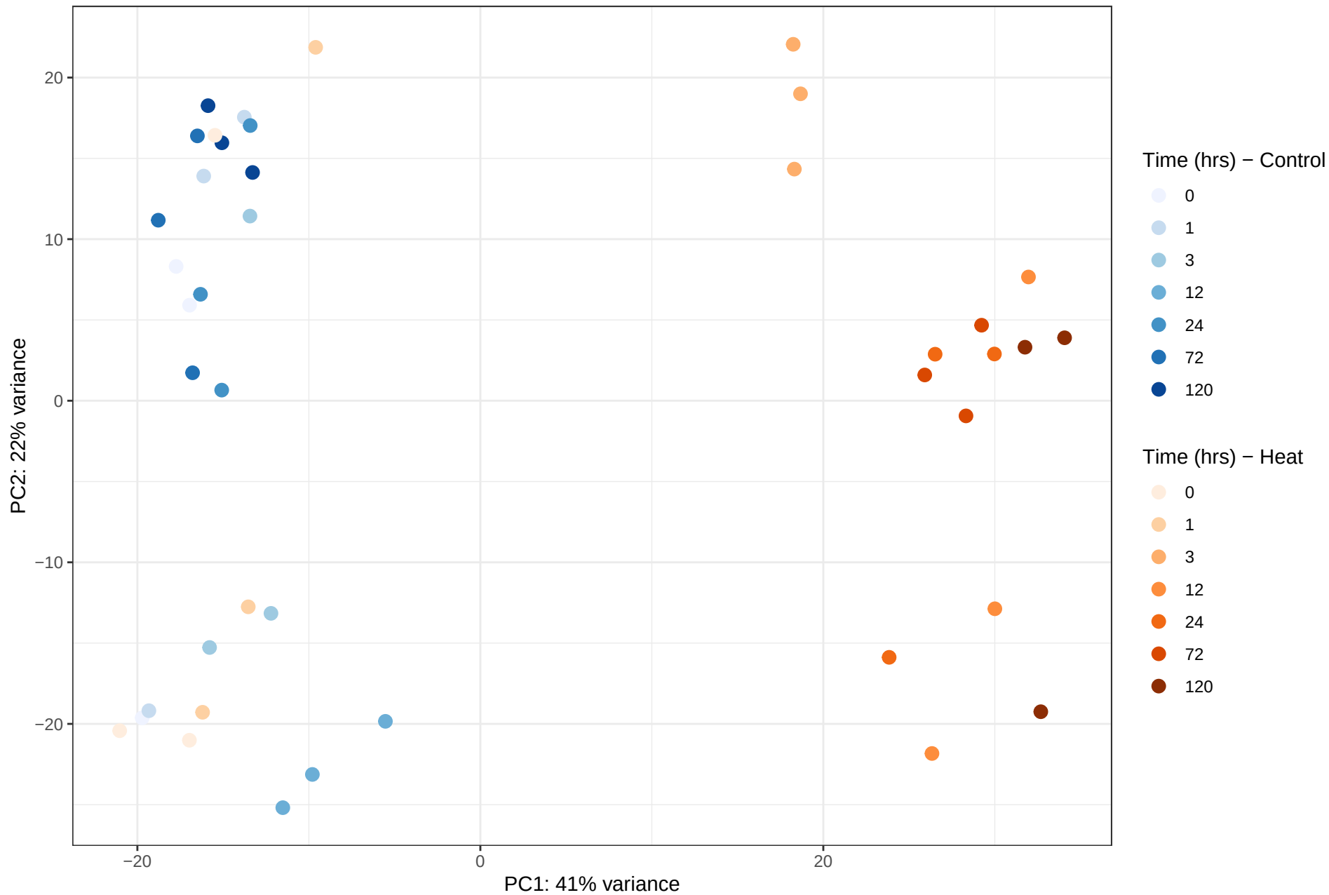
Pacuta – PCA of VST-transformed counts
