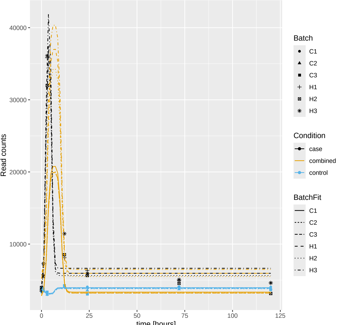
Pocillopora_acuta_Hlv2____RNAseq.g26418.t1: log10 q = -84.86
