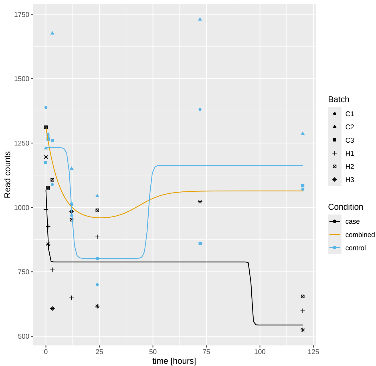
Montipora_capitata_Hlv3___RNAseq.g45122.t1: log10 q = -2.42
