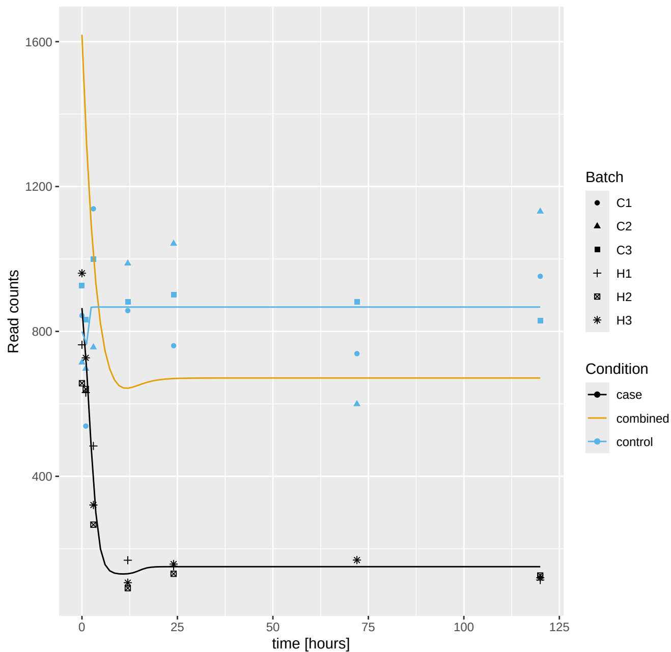
Montipora_capitata_Hlv3___RNAseq.g40931.t1: log10 q = -33.07
