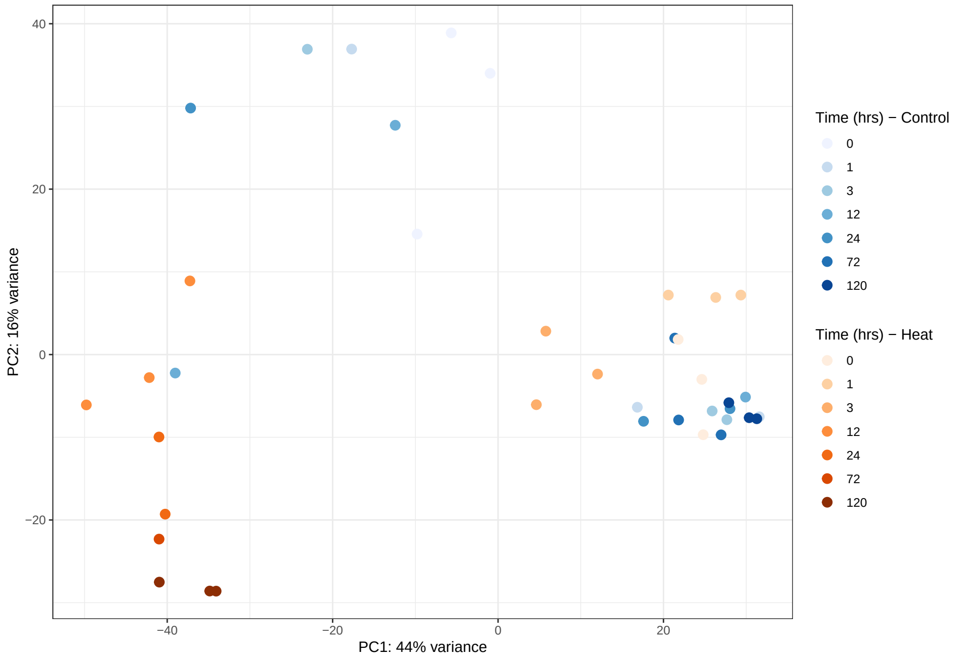
Pcomp – PCA of VST-transformed counts
